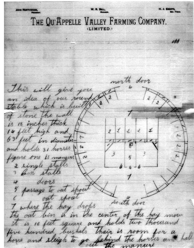
Plan of the Bell Barn drawn by Guy May on December 25, 1882, showing location of the stalls and bins.
